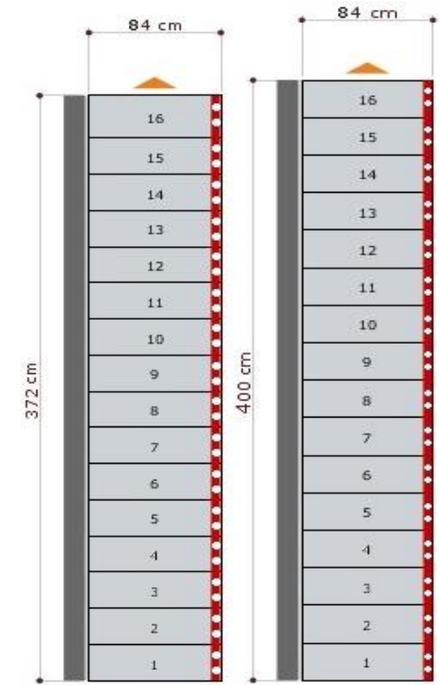
230mm Goings 250mm Goings 16 Tread Composity
