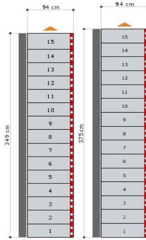
230mm Goings 250mm Goings 15 Tread Composity
