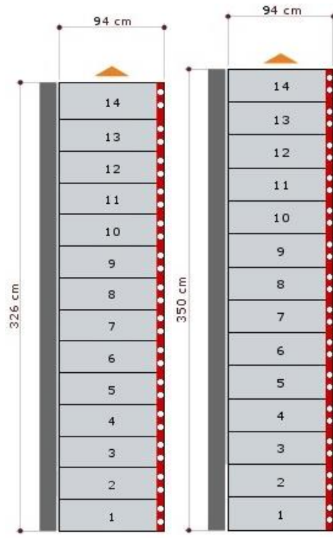
230mm Goings 250mm Goings 14 Tread Composity
