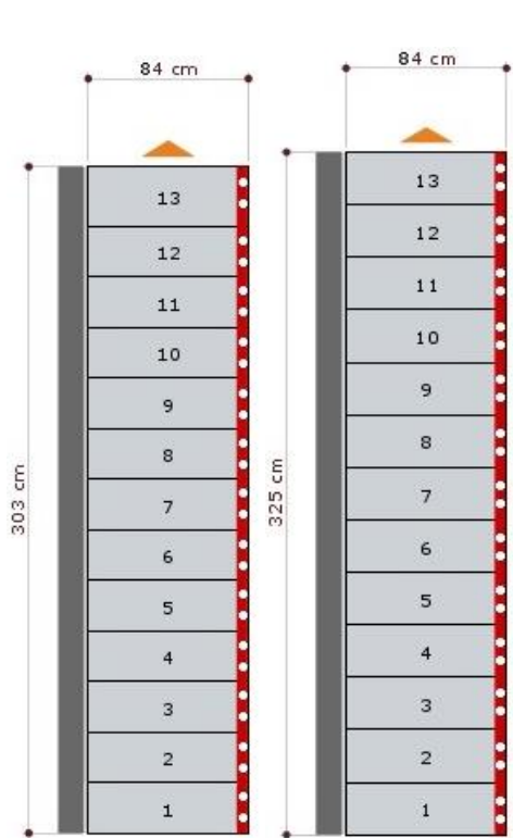
230mm Goings 250mm Goings 13 Tread Composity
